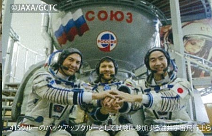
©JAXA/GTC
